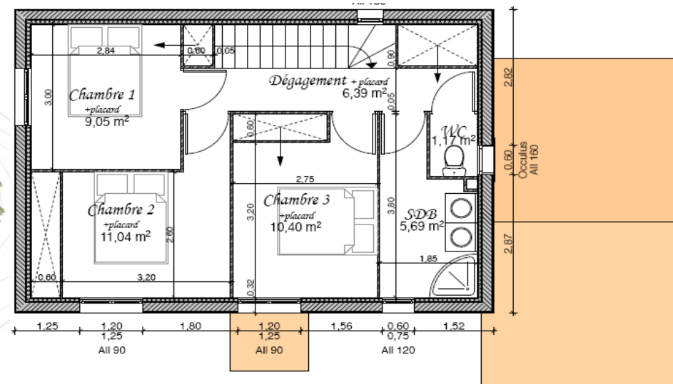
Plan R+1
